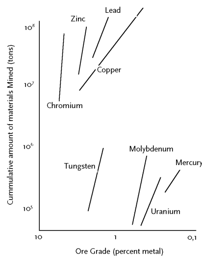
Figure 9: The relation between the availability of resources and the ore grade on a logarithmic scale for a number of minerals. A steep line indicates that the availability increases sharply if mankind is able and willing to accept a slightly lower ore concentration. A flat line means that even at lower concentrations, the availability will not increase very much. The latter case is more problematic than the first. [Taken from Chapman 83]
