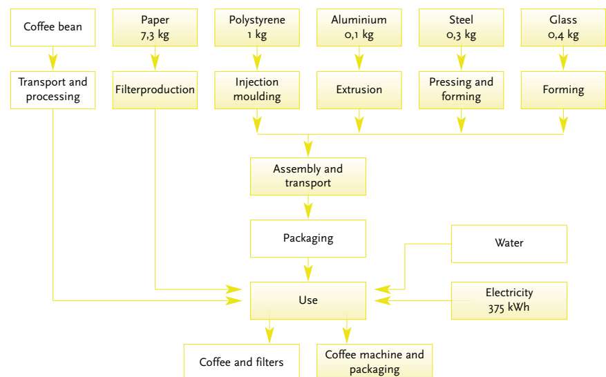
Figure 3: Process tree of a simplified coffee machine model with amounts and assumptions. White boxes are not included in the analysis.
