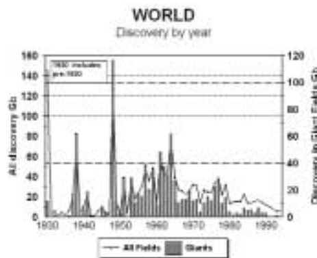
Figure 10: The discovery rate of liquid oil has dropped to an average of about 6 Gigabarrel per year, while the extraction is almost tenfold. The so-called giant fields have all been discovered during the fifties, sixties and seventies. The present knowledge of geology is so well developed that it is unlikely that many new giant fields can be found.
